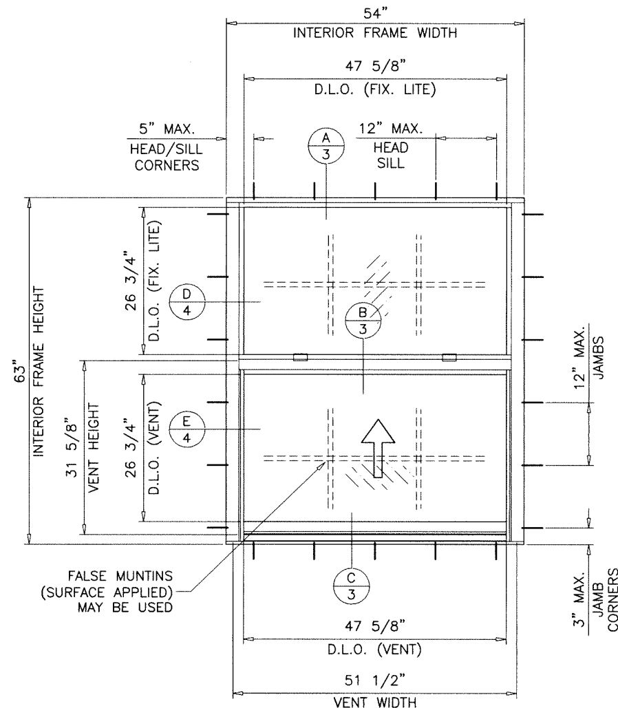
TYPICAL ELEVATION EQUAL LITES
